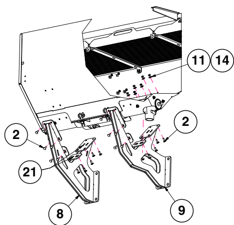
Tank Mounts
