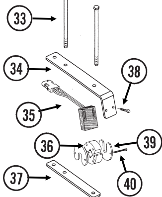
Shaft Rotation Sensor
