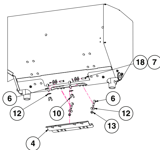
Clean-Out Doors
