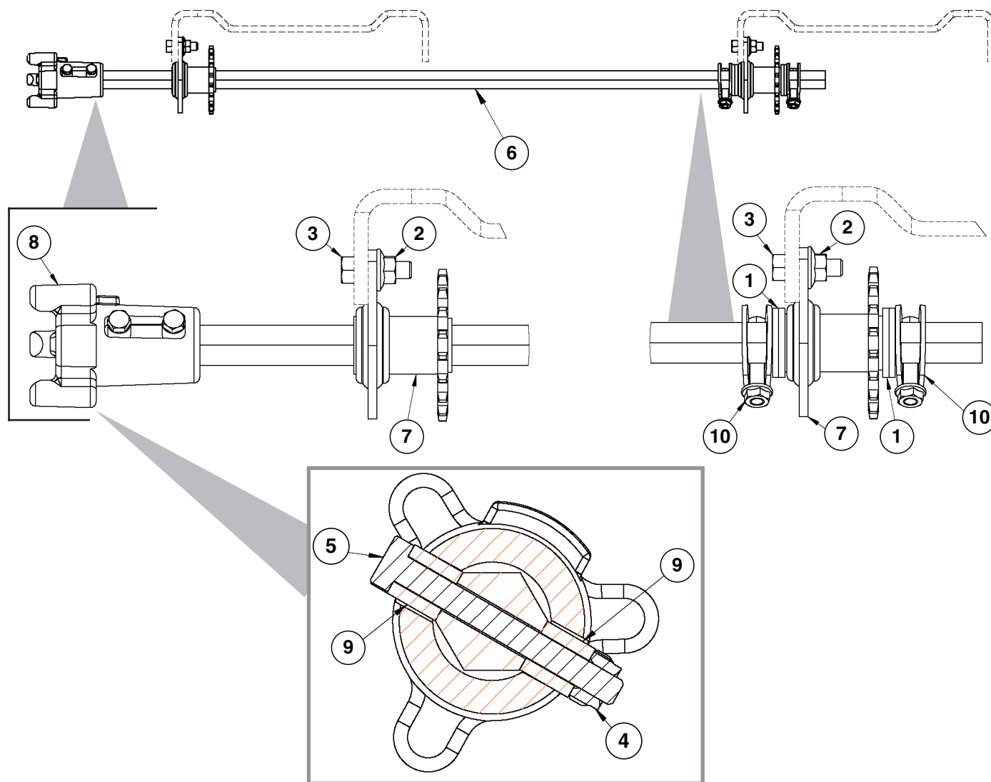
Coupler Cross-Section
