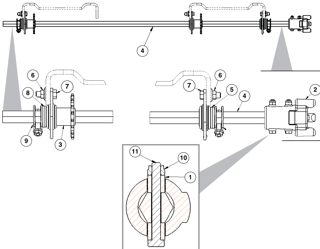
Coupler Cross-Section
