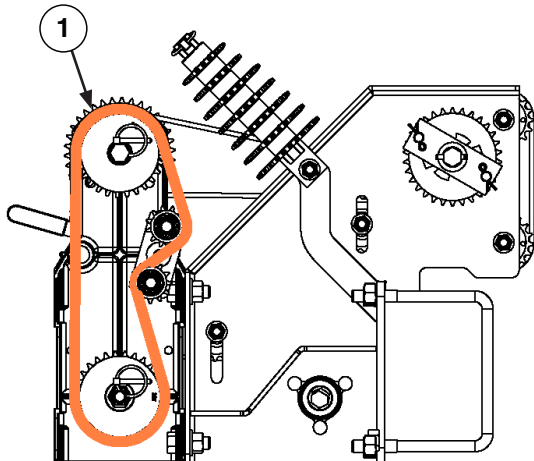
L.H. View of Transmission
