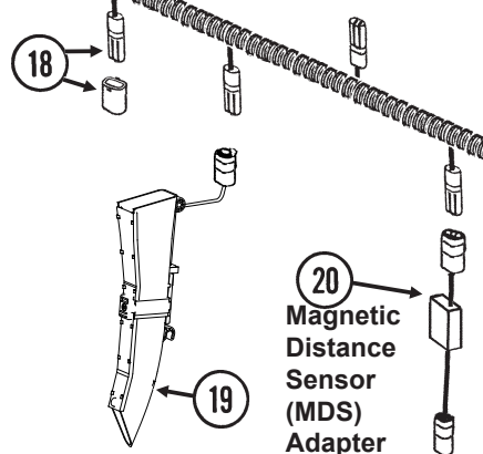
Planter Harness
