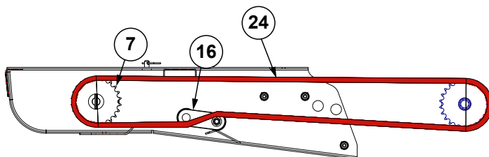
Chain Routing
