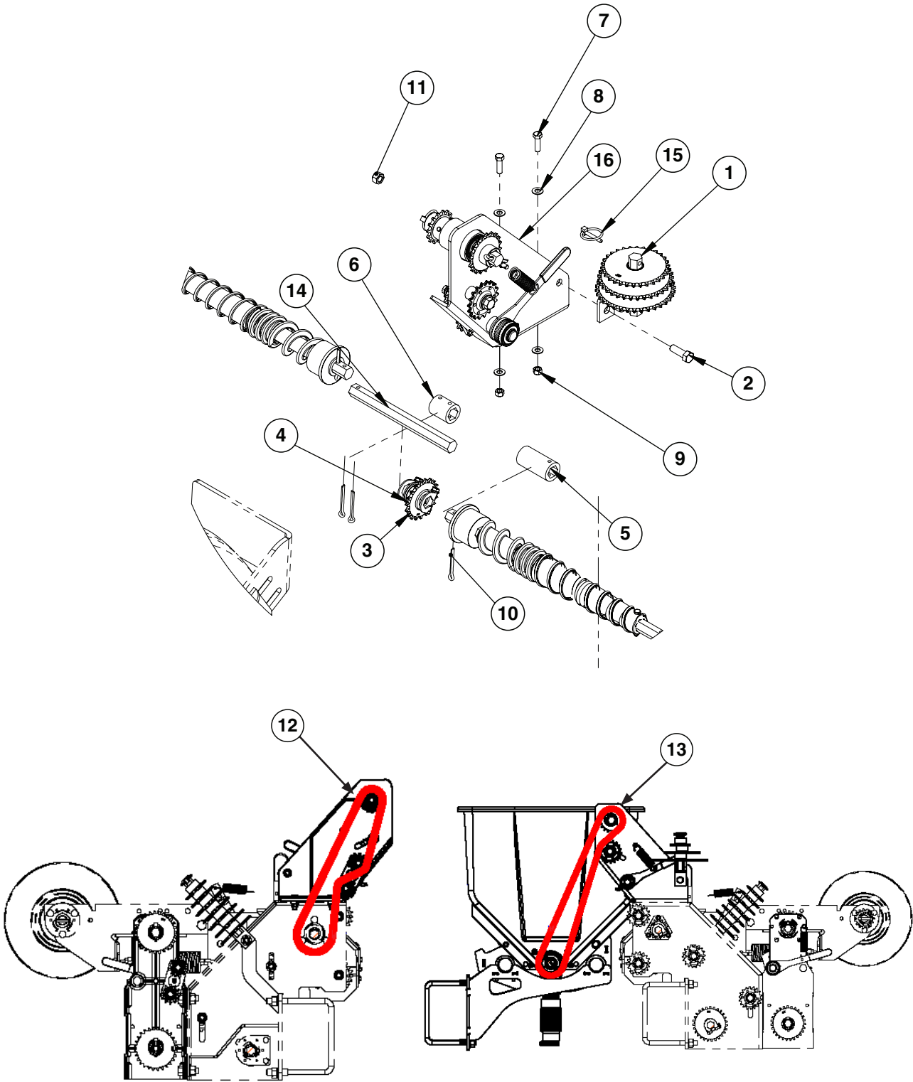
Transmission Side View (Both Sides)
