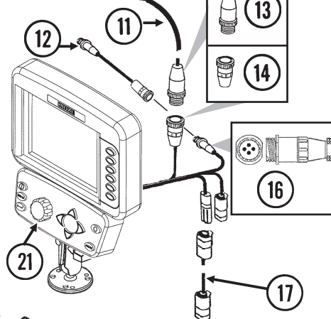
Power Lead Adapter
