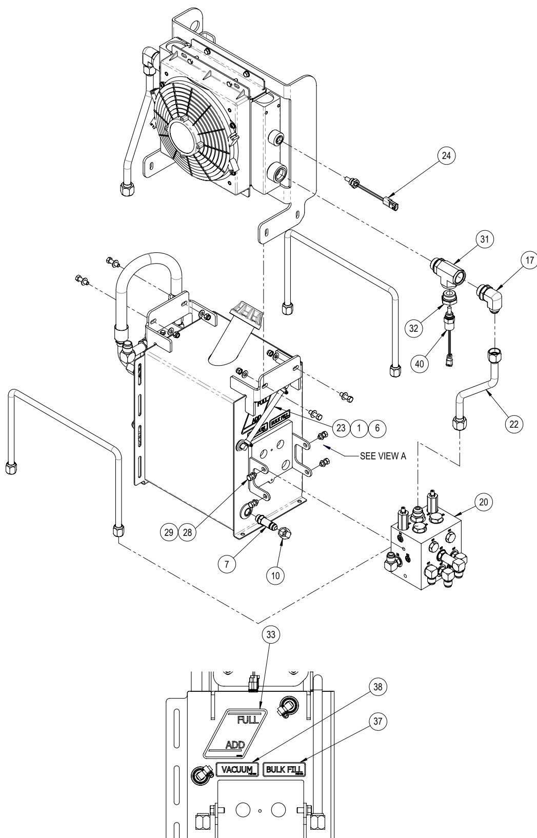
VIEW A
