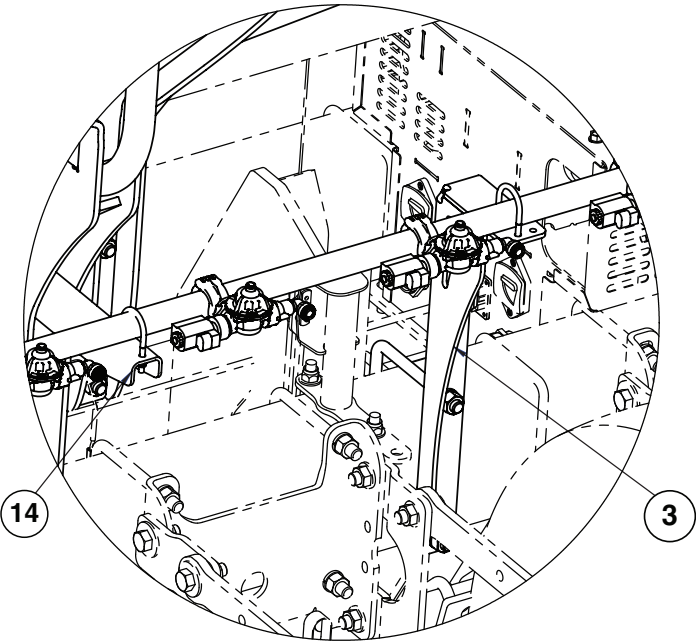
DETAIL A
