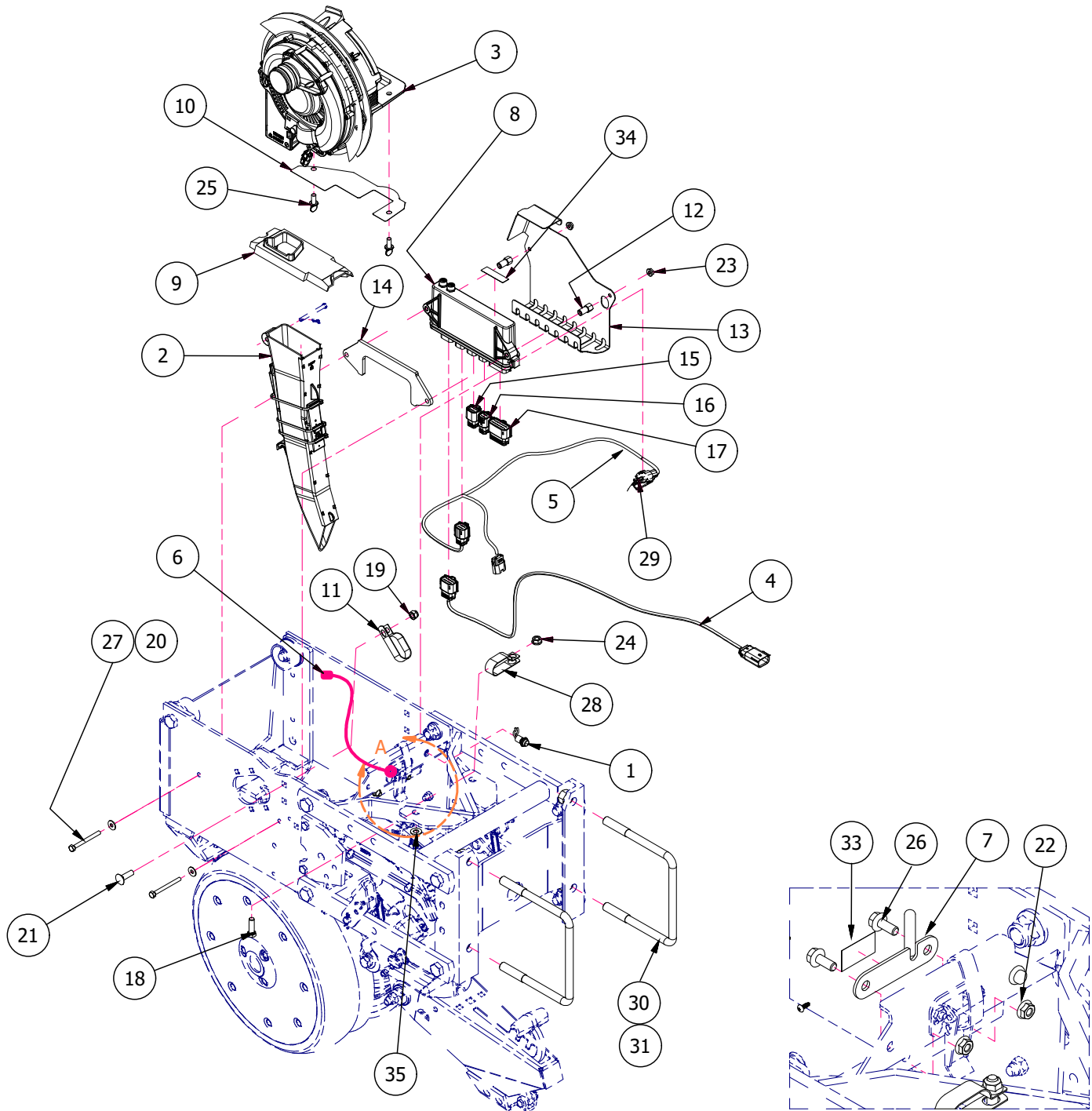
VIEW A
