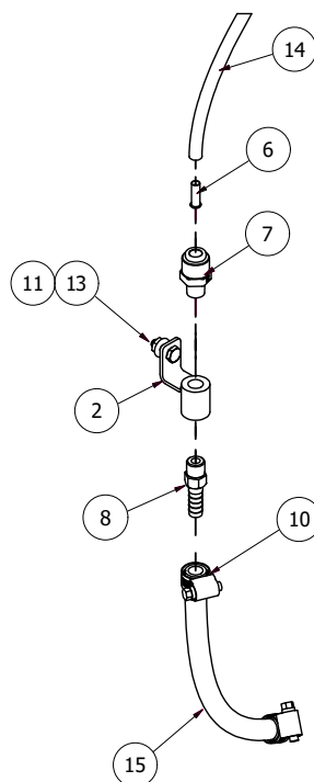
DETAIL B
