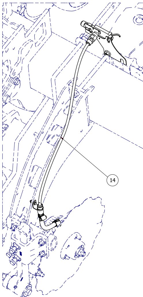
DETAIL A
