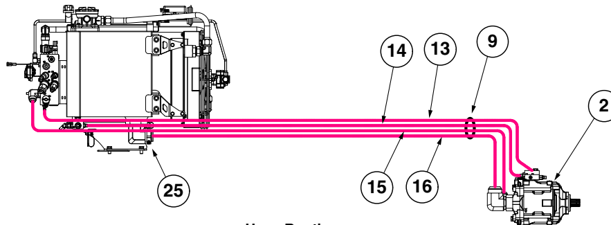
Hose Routing
