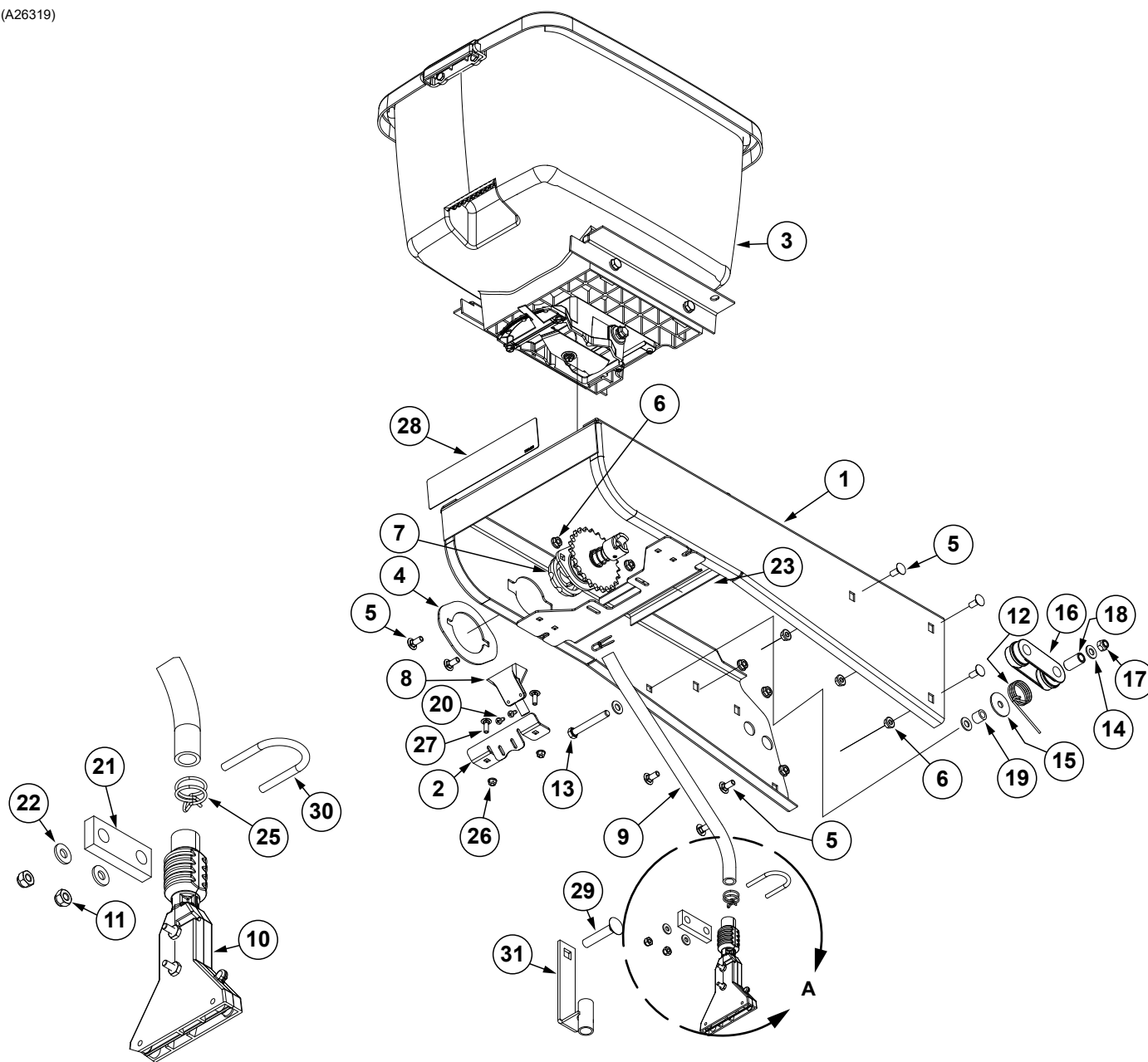
Detail A
