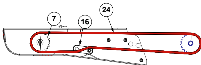
Chain Routing
