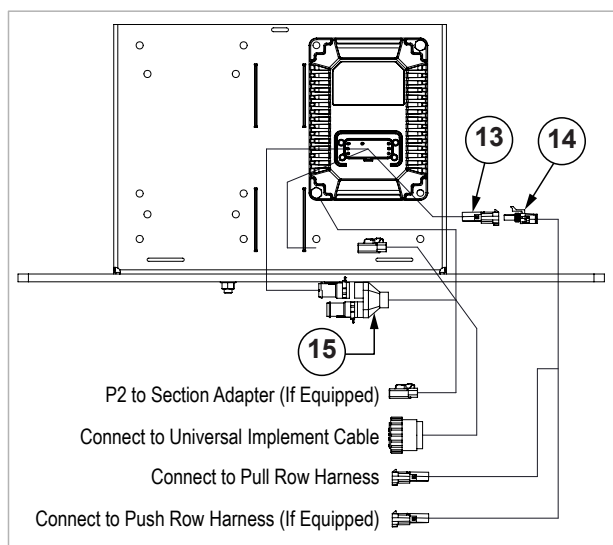
Wire Diagram
