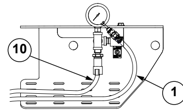
PDP Air Supply W/Yetter Electric Compressor (16 Row Shown)
