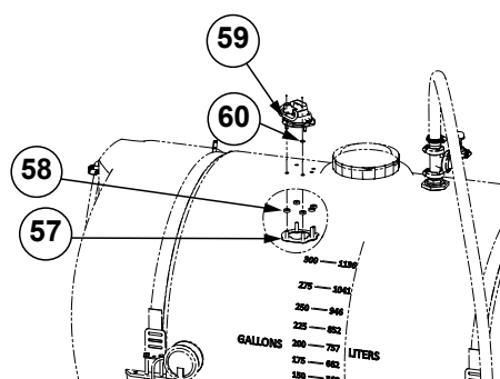
View H (2 Places)
