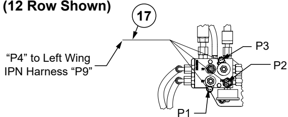
Harness Routing
