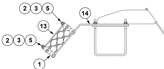
View D (16 Row)
