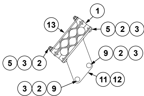
View J (16 Row)
