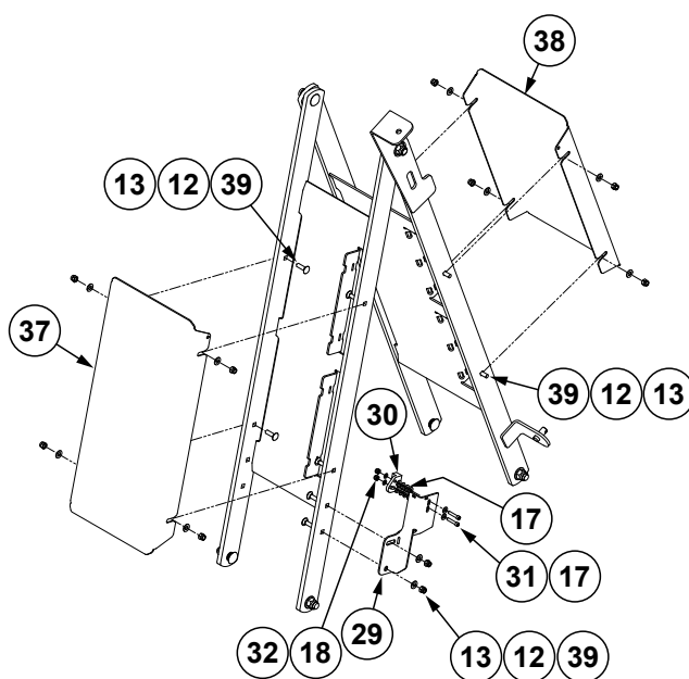
Detail G 16 Row
