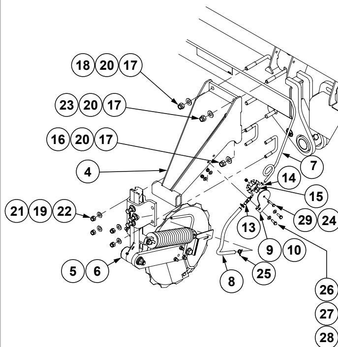
Wide (Wing Hinge) (L.H. Shown)
