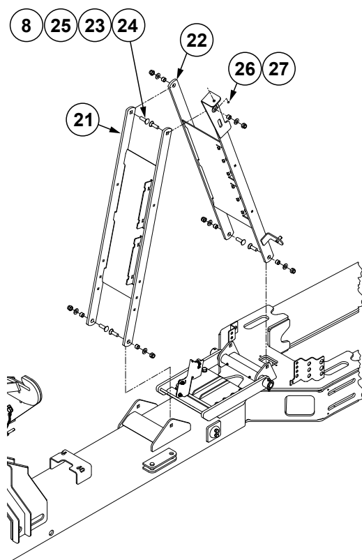
Detail F
