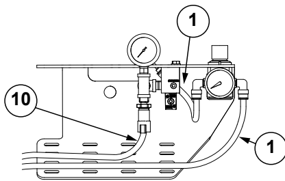
PDP Air Supply W/Yetter Air Compressor (16 Row Shown)
