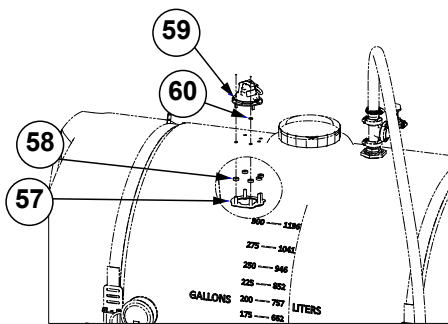
View G (2 Places)
