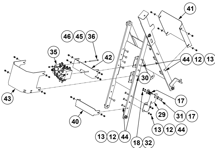
Detail H 12 Row
