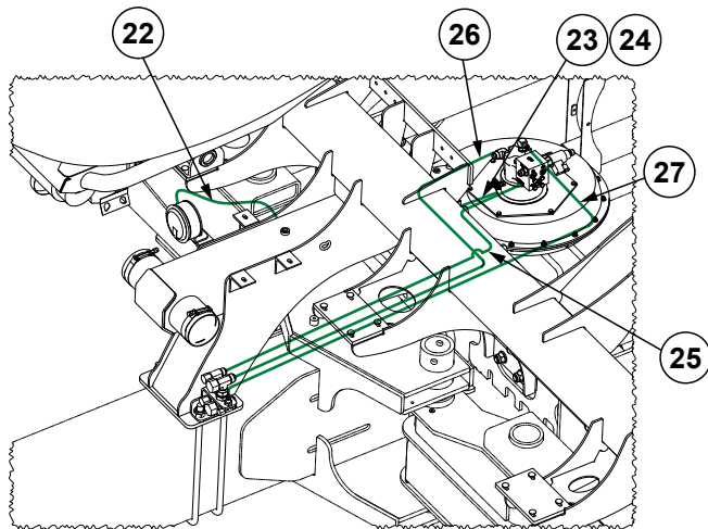
Hose Routing
