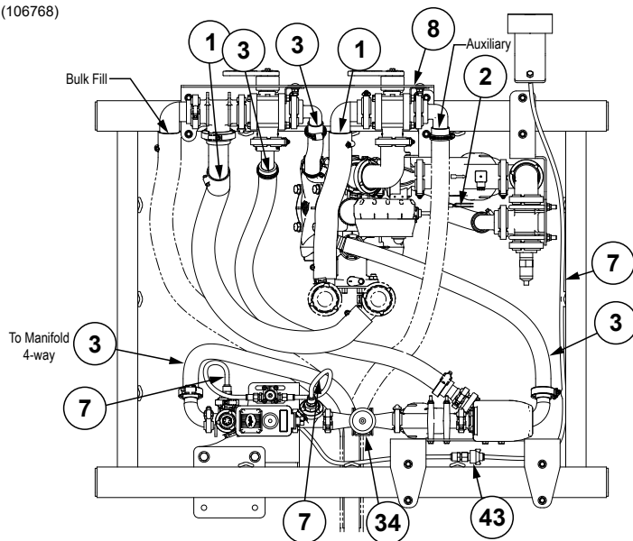
Hose Routing with Auxiliary
