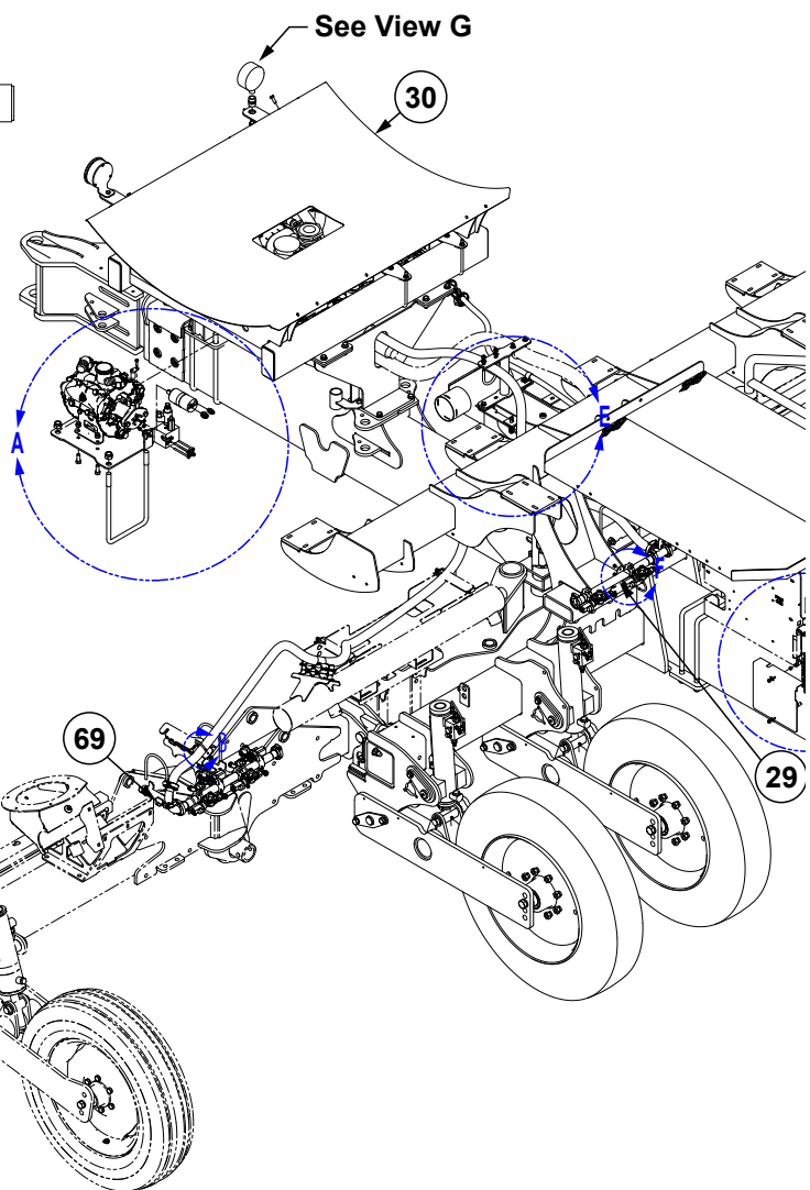
Hose Routing with Auxiliary
