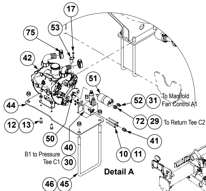
Hose Routing with Auxiliary
