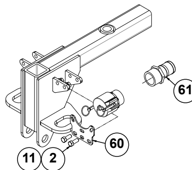
Rear Trailer Hitch Option
