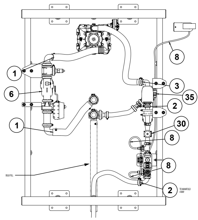
Hose Routing without Aux
