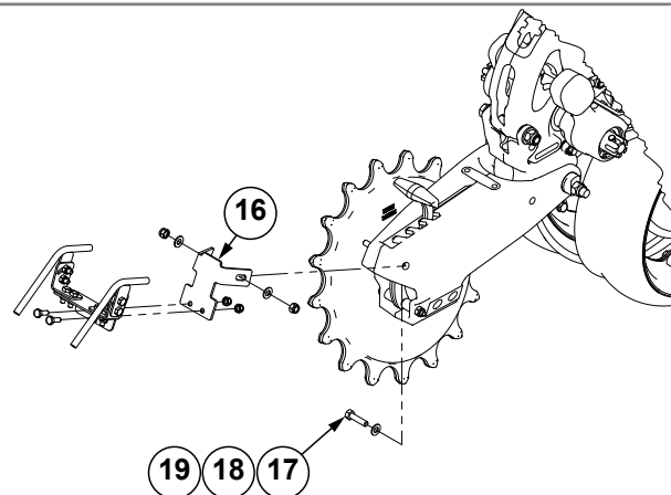
Spring Closing Wheels
