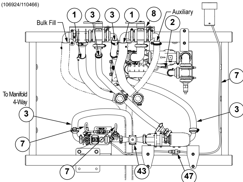
Hose Routing with Auxiliary (2024-2025 Production)
