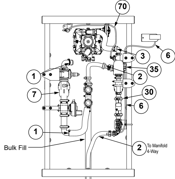
Hose Routing without Auxiliary
