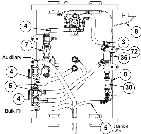
Hose Routing with Auxiliary
