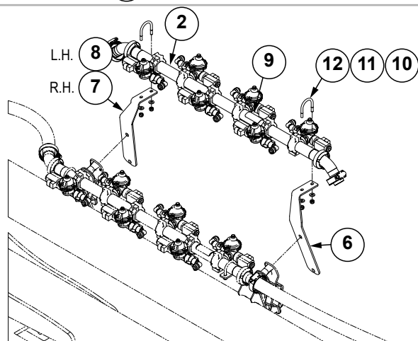
View H (Inner Wing Manifolds)
