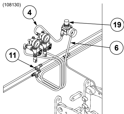
Air Closing Wheel Air Supply W/Yetter Compressor and No PDP
