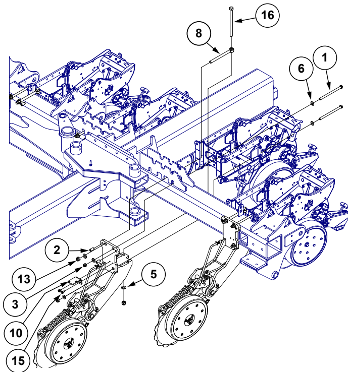
Extended Mount
