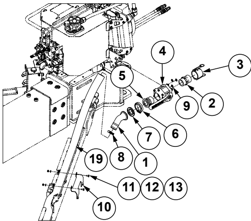
Front Hitch
