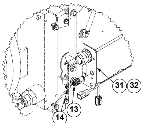
View H-H (View Reoriented for Clarity)
