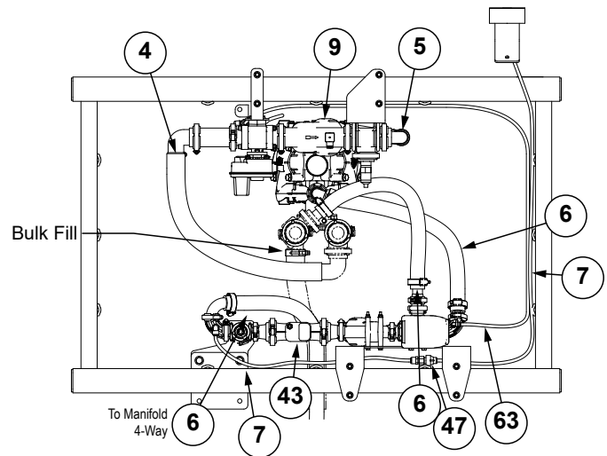
Hose Routing without Auxiliary
