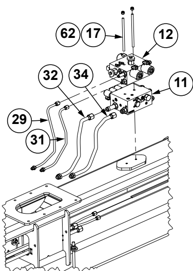
L.H. Wing Hydraulic Block Detail
