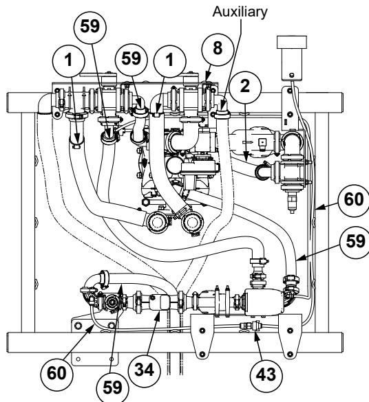
Hose Routing with Auxiliary
