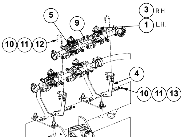
View G (Outer Wing Manifolds)
