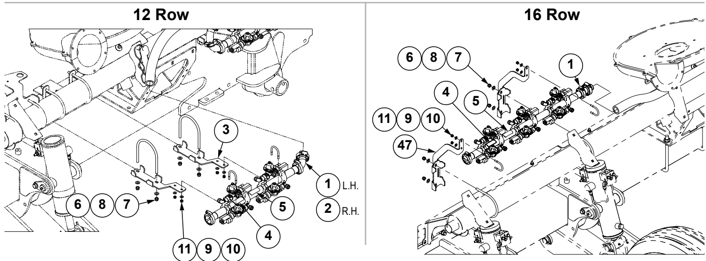
View G (Wing Manifolds)
