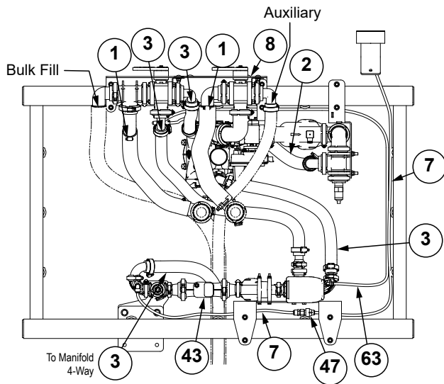
Hose Routing with Auxiliary
