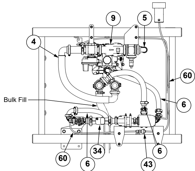
Hose Routing without Auxiliary
