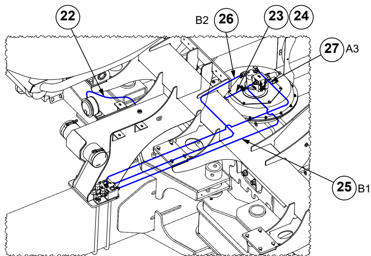
View D Hose Routing (Some parts not shown for clarity)
