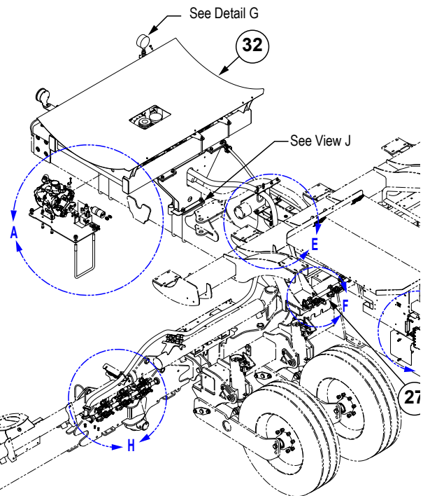
Hose Routing with Auxiliary (2024-2025 Production)
