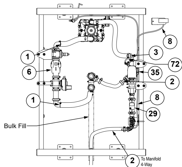
Hose Routing without Auxiliary
