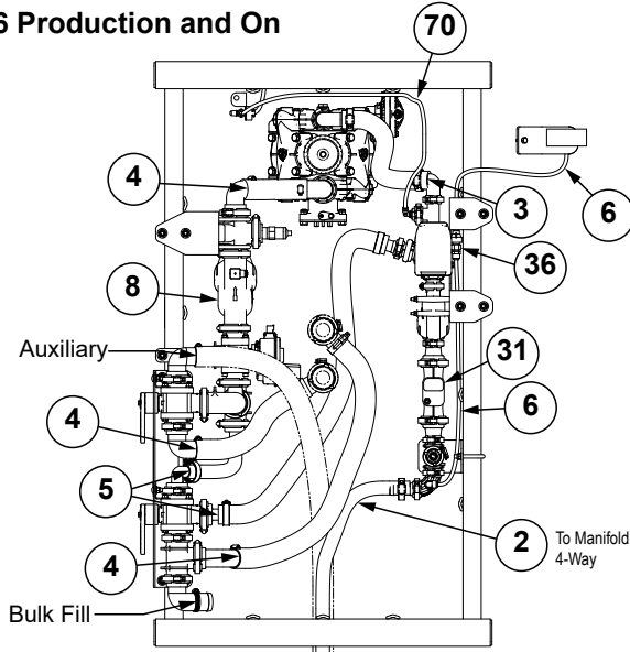
Hose Routing with Auxiliary
