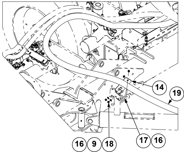
R.H. Draft Link Pivot - 12 Row and 16 Row
