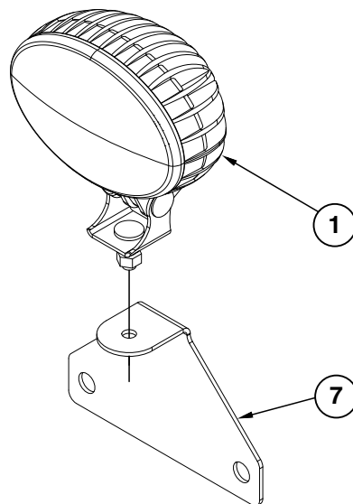
Work Light
