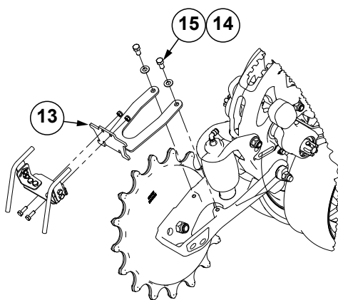
Air Closing Wheels
