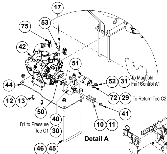
Hose Routing with Auxiliary (2024-2025 Production)
