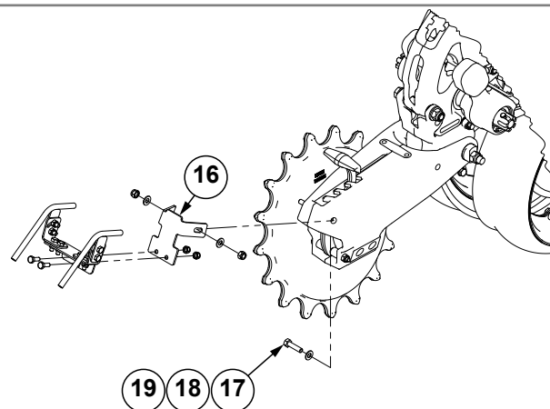
Spring Closing Wheels
