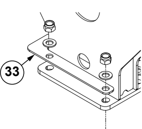
Detail F
