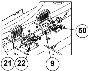
View E (Center Frame Manifolds)
