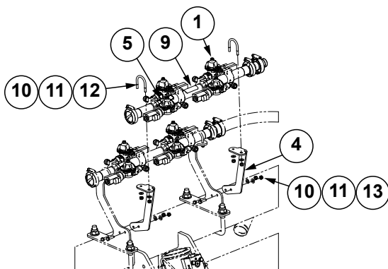
View G (Outer Wing Manifolds)
