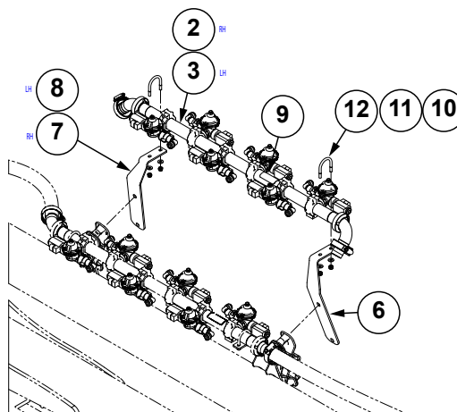
View H (Inner Wing Manifolds)
