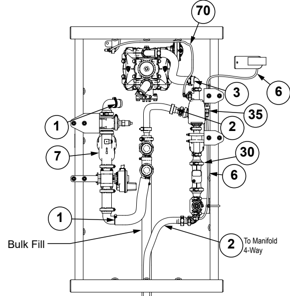
Hose Routing without Auxiliary
