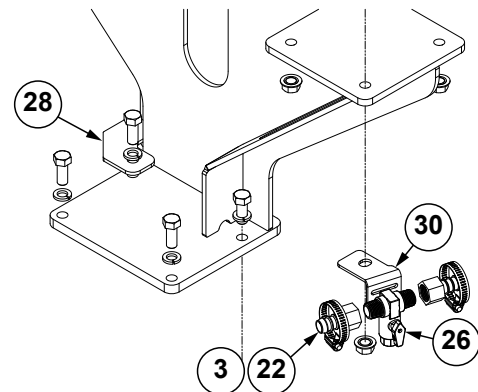
Detail G
